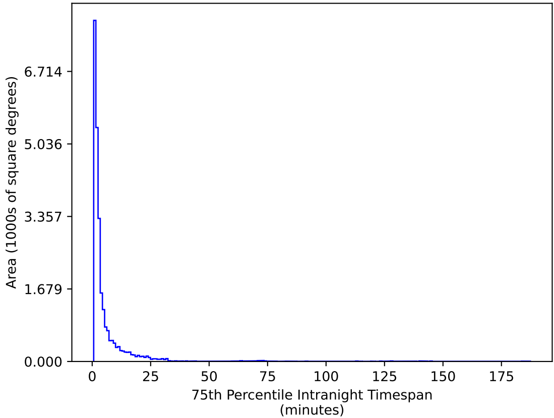
ddf_loaded_fl15_v3.4_10yrs All sky g band: 75th Percentile Intranight Timespan
