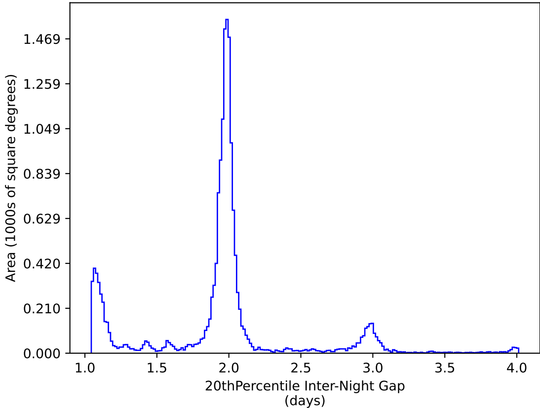
ddf_loaded_fl15_v3.4_10yrs WFD y band: 20thPercentile Inter-Night Gap
