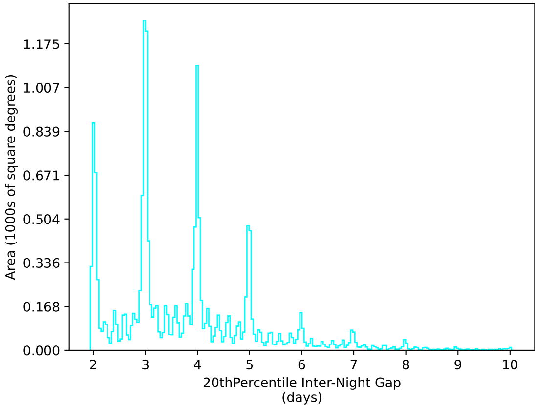
ddf_loaded_fl15_v3.4_10yrs WFD u band: 20thPercentile Inter-Night Gap
