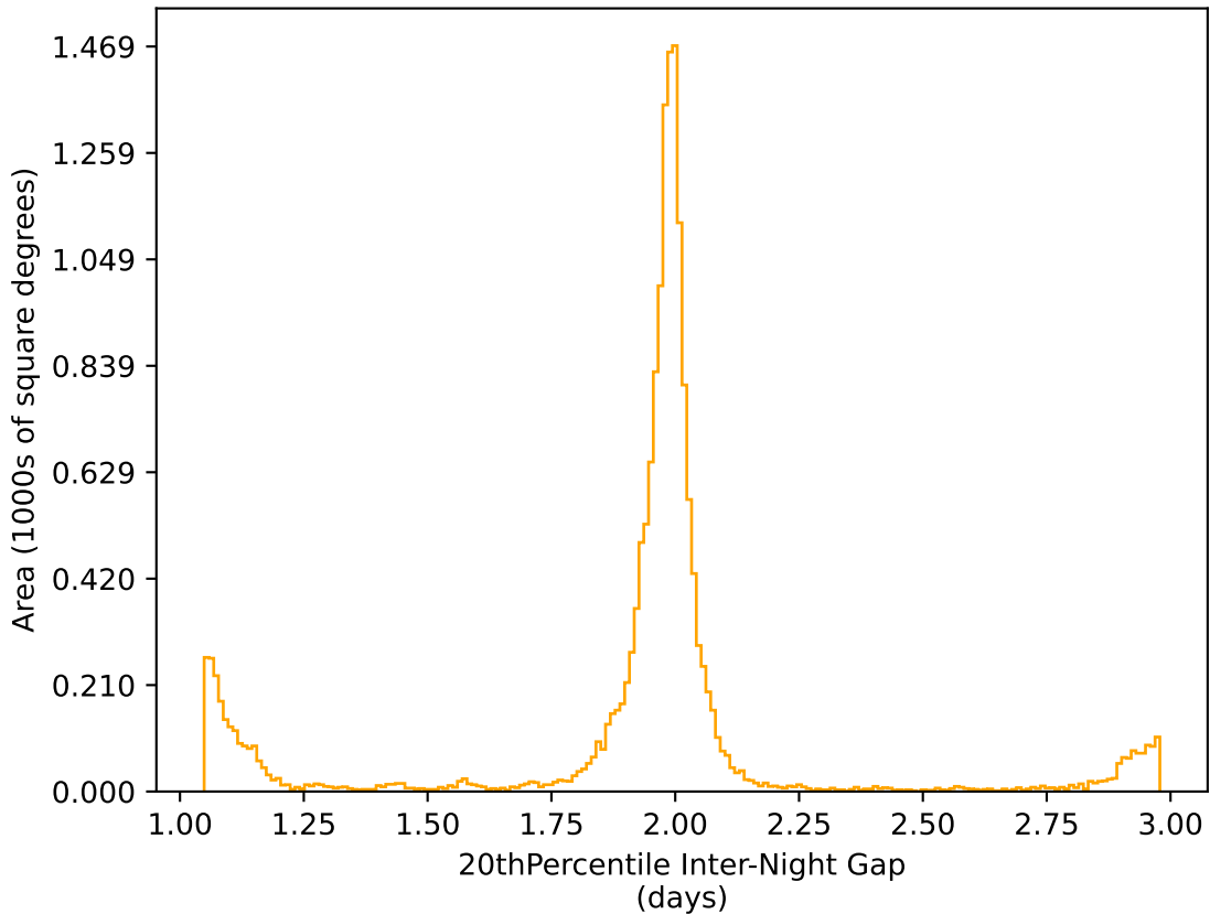
ddf_loaded_fl15_v3.4_10yrs WFD r band: 20thPercentile Inter-Night Gap
