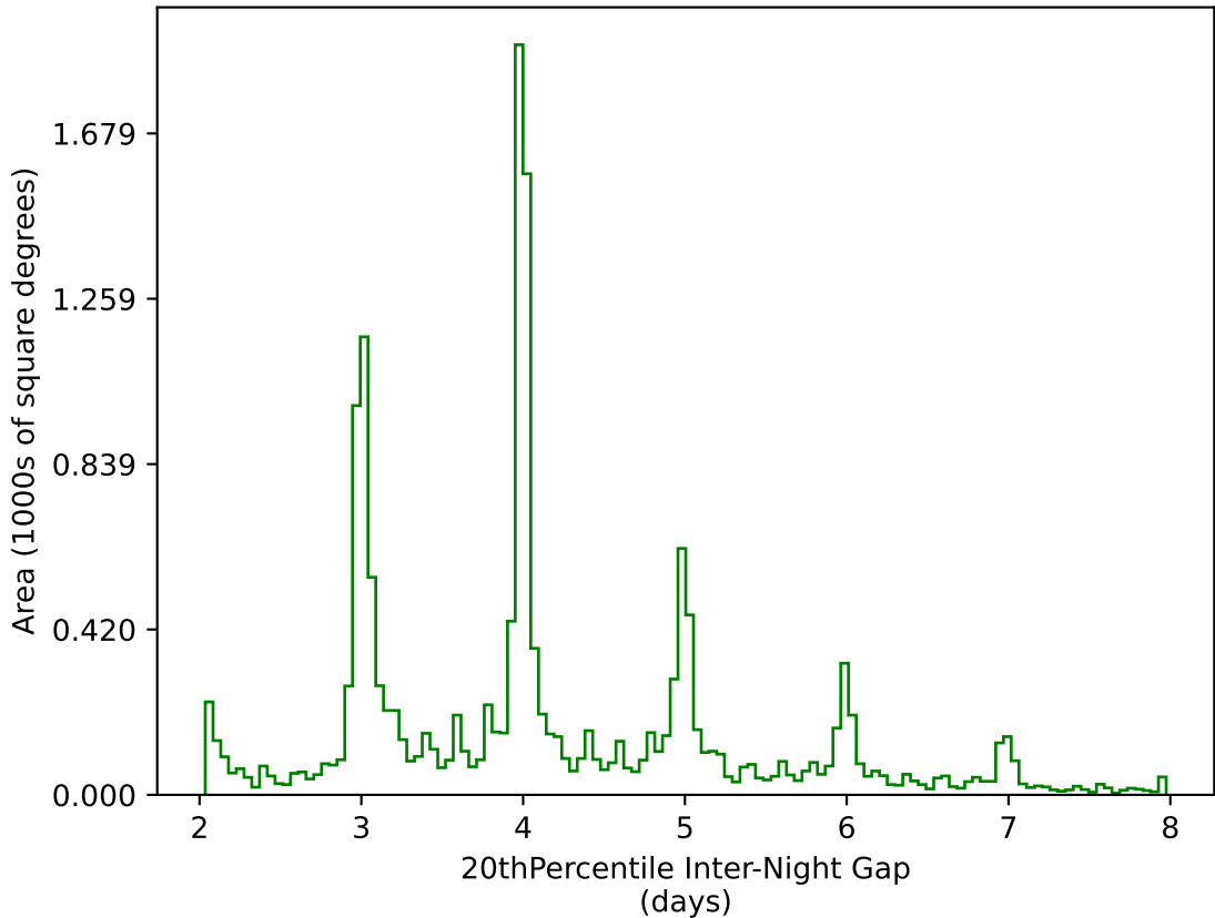
ddf_loaded_fl15_v3.4_10yrs WFD g band: 20thPercentile Inter-Night Gap
