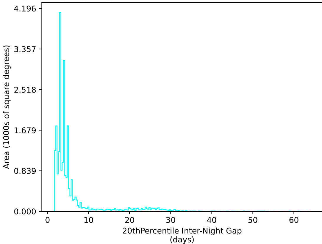
ddf_loaded_fl15_v3.4_10yrs All sky u band: 20thPercentile Inter-Night Gap
