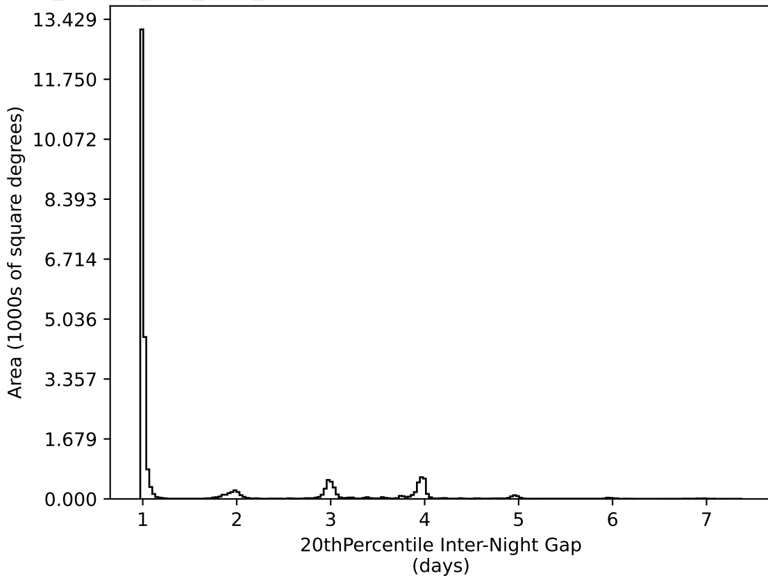
ddf_loaded_fl15_v3.4_10yrs All sky all bands: 20thPercentile Inter-Night Gap
