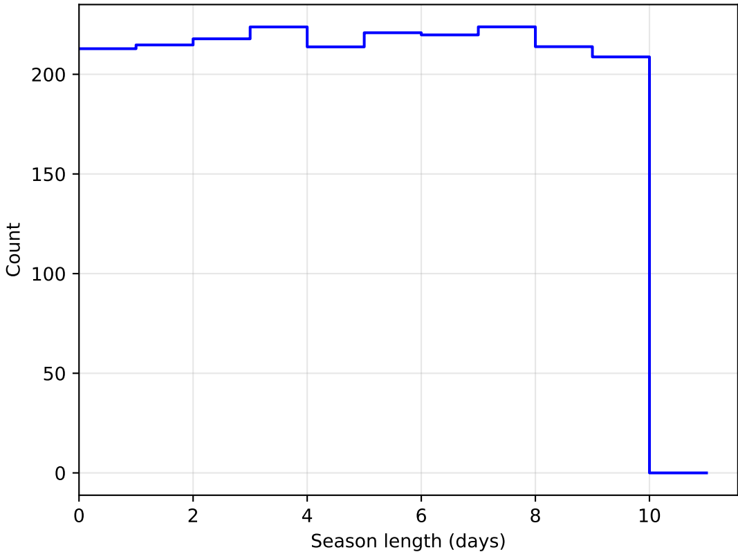
ddf_loaded_fl15_v3.4_10yrs DD:EDFS all bands: SeasonLength
