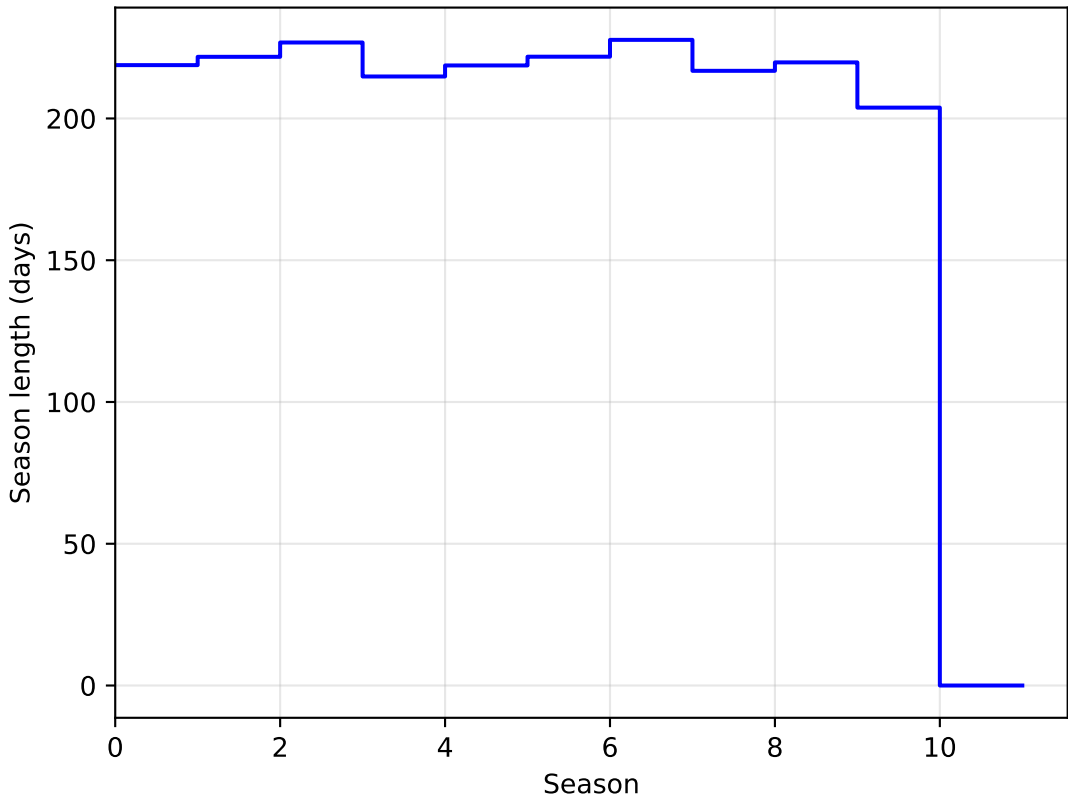
ddf_loaded_fl15_v3.4_10yrs DD:ECDFS all bands: SeasonLength
