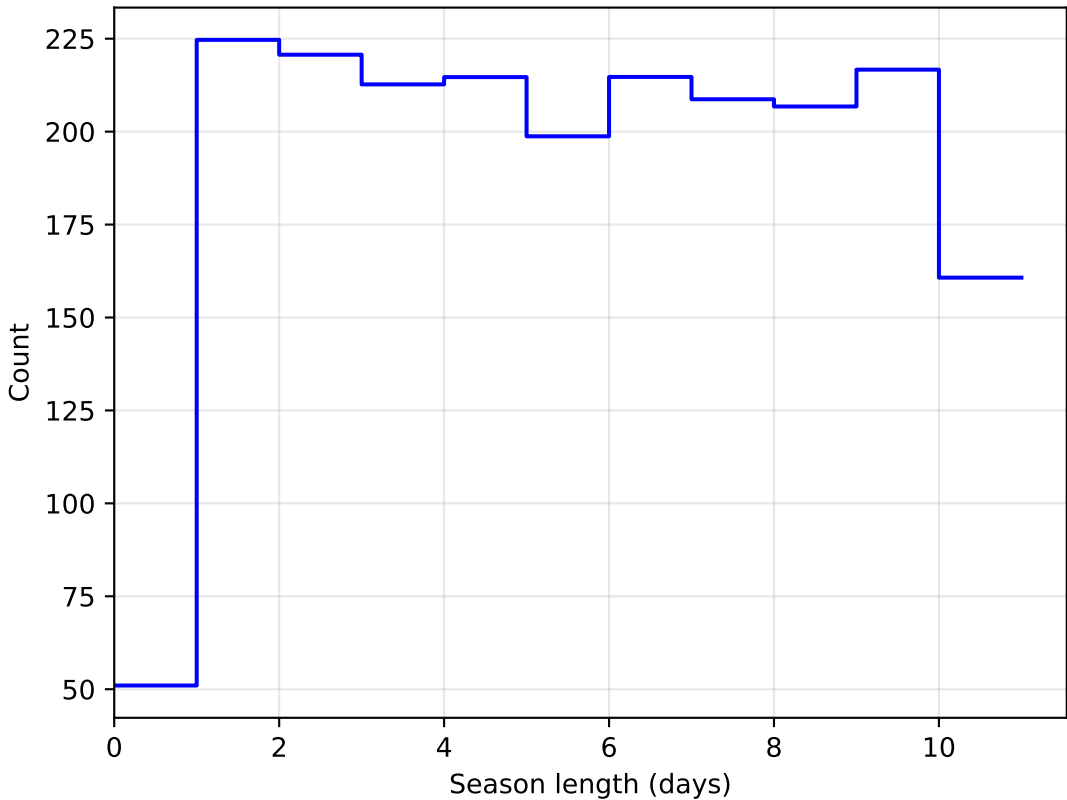
ddf_loaded_fl15_v3.4_10yrs DD: COSMOS all bands: SeasonLength
