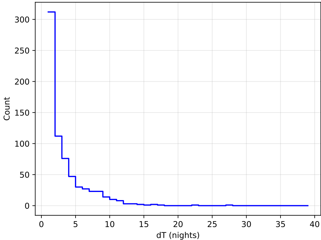
ddf_loaded_fl15_v3.4_10yrs all bands: DD:XMM_LSS Delta Nights Histogram
