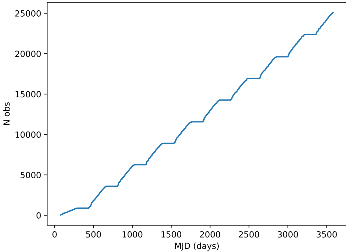
ddf_loaded_fl15_v3.4_10yrs all bands: DD:XMM_LSS Cumulative NVisits
