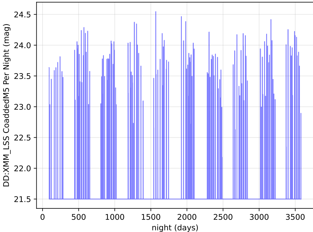
ddf_loaded_fl15_v3.4_10yrs y band: DD:XMM_LSS CoaddedM5 Per Night
