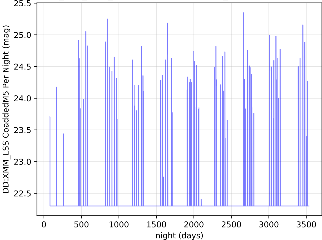
ddf_loaded_fl15_v3.4_10yrs u band: DD:XMM_LSS CoaddedM5 Per Night
