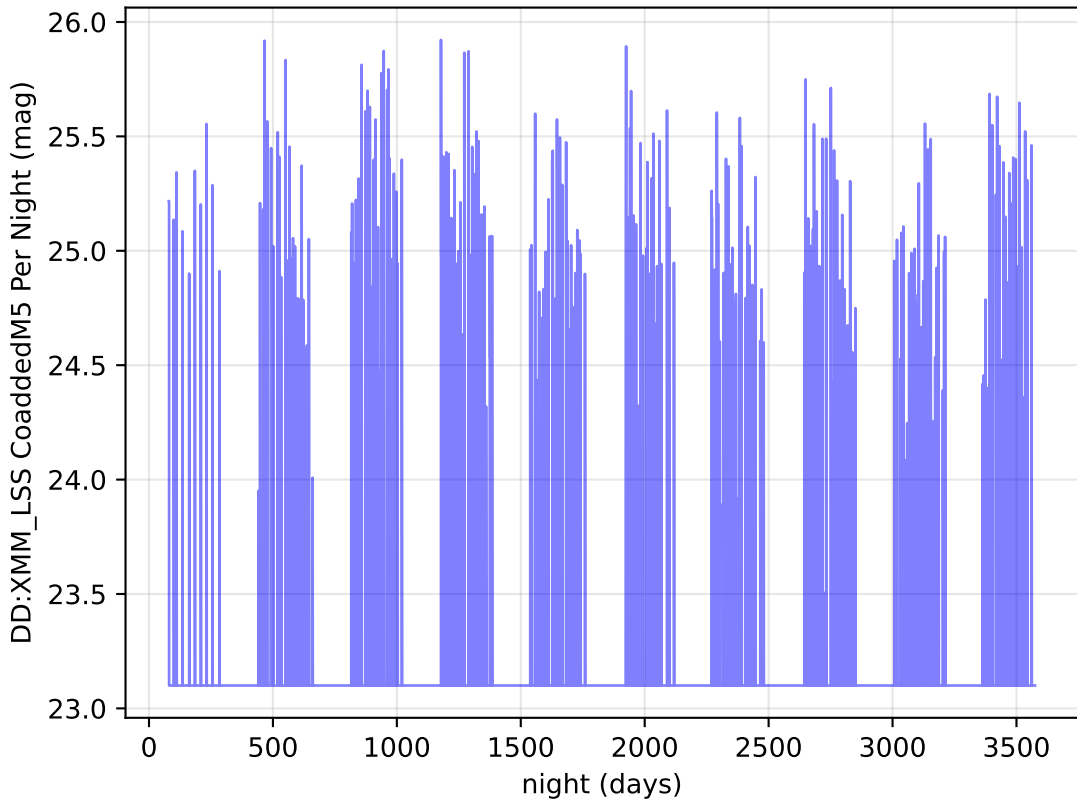
ddf_loaded_fl15_v3.4_10yrs i band: DD:XMM_LSS CoaddedM5 Per Night
