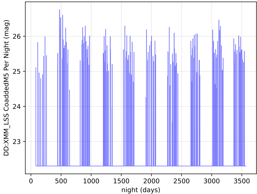
ddf_loaded_fl15_v3.4_10yrs g band: DD:XMM_LSS CoaddedM5 Per Night
