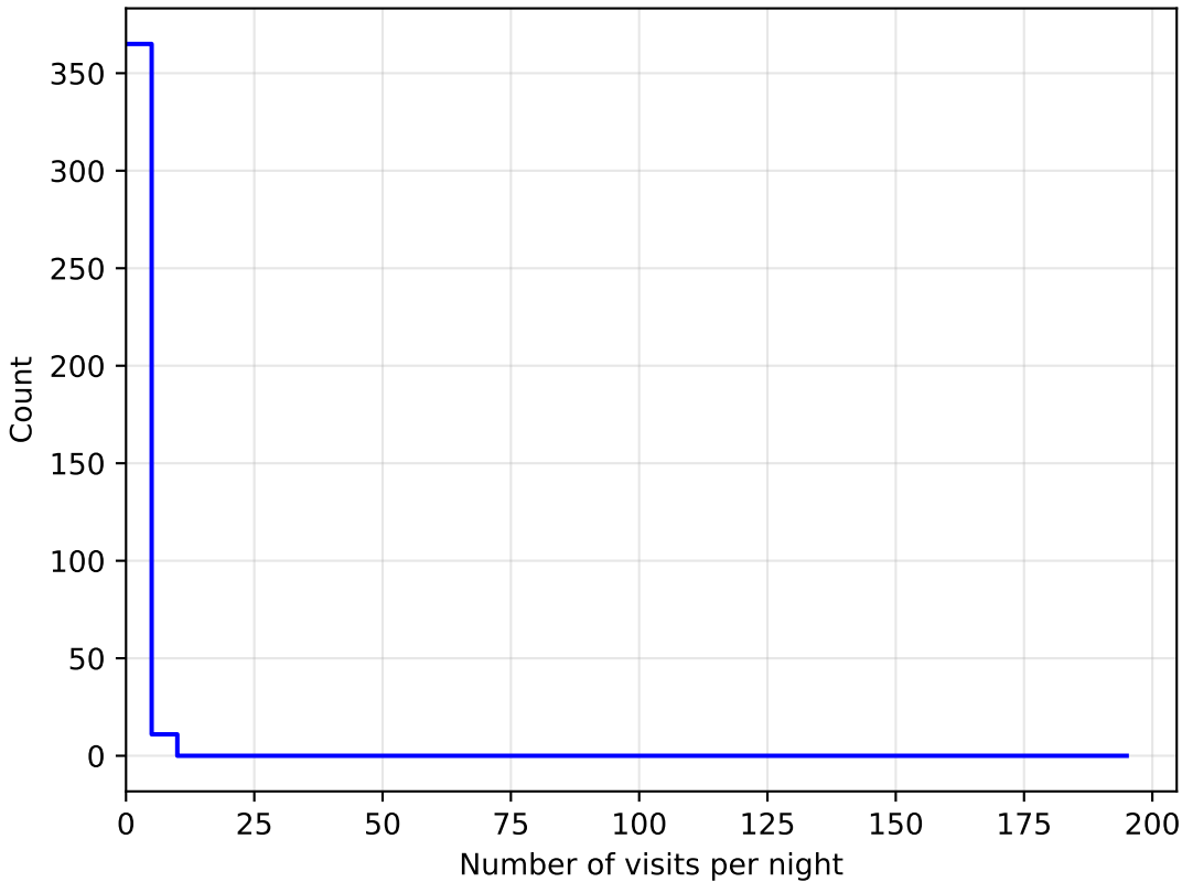
ddf_loaded_fl15_v3.4_10yrs all bands: DD:WFD NVisitsPerNight
