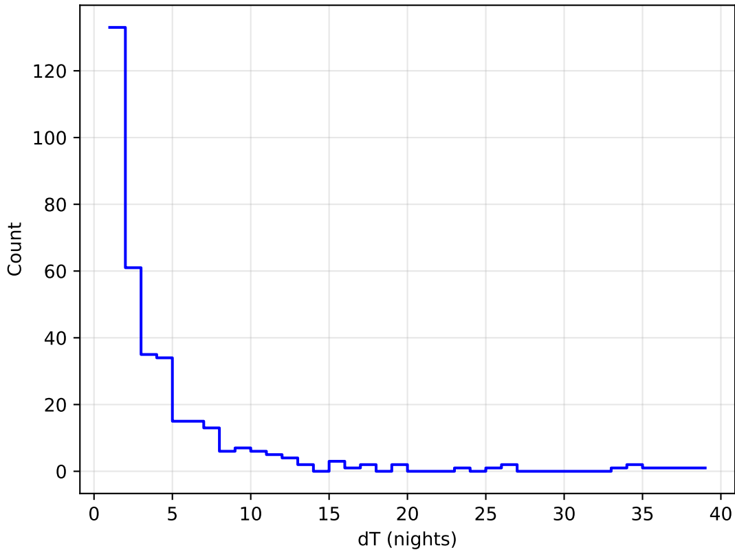
ddf_loaded_fl15_v3.4_10yrs all bands: DD:WFD Delta Nights Histogram
