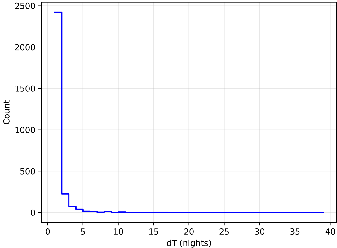
ddf_loaded_fl15_v3.4_10yrs all bands: DD:WFD Delta Nights Histogram
