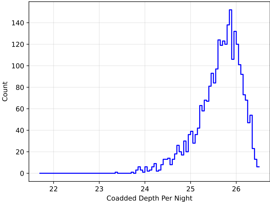
ddf_loaded_fl15_v3.4_10yrs z band: DD:WFD CoaddM5PerNight
