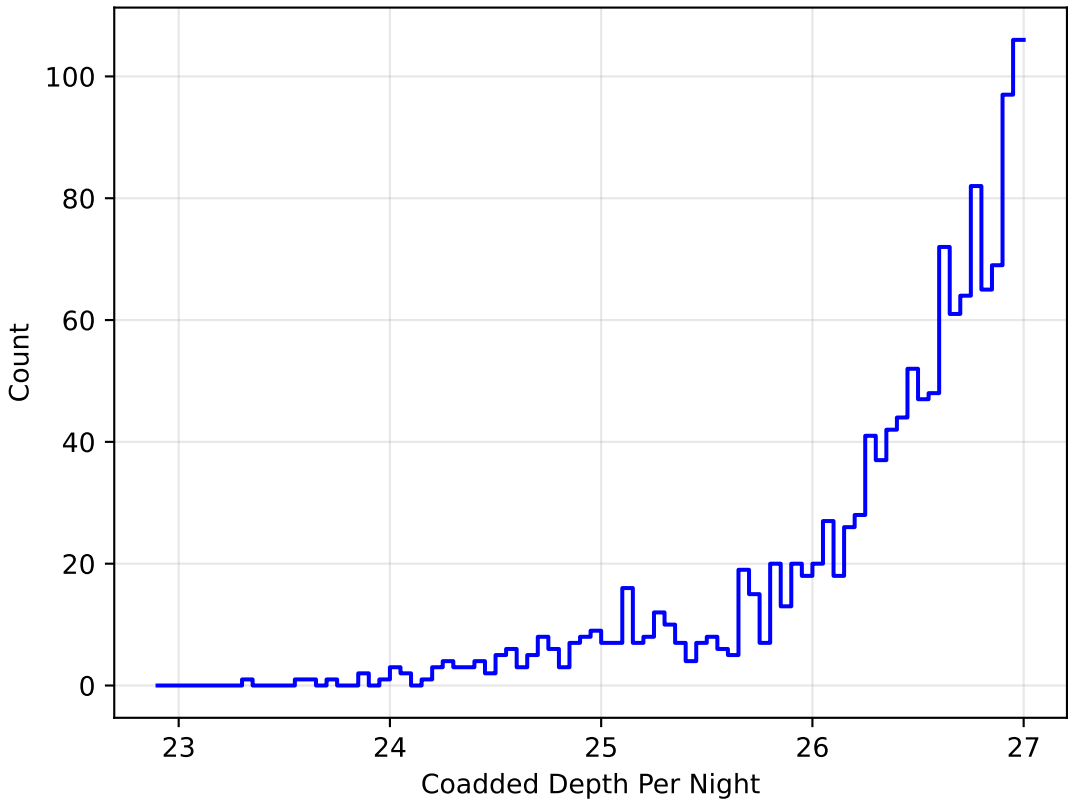
ddf_loaded_fl15_v3.4_10yrs r band: DD:WFD CoaddM5PerNight
