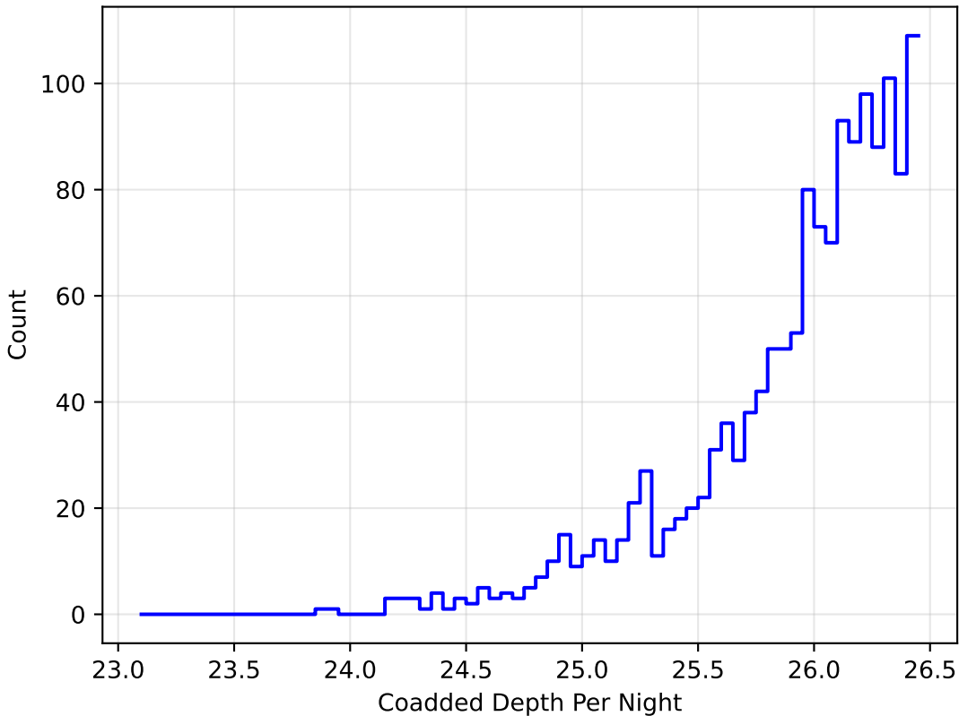
ddf_loaded_fl15_v3.4_10yrs i band: DD:WFD CoaddM5PerNight
