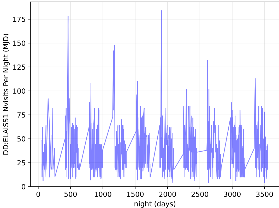
ddf_loaded_fl15_v3.4_10yrs all bands: DD:ELAISS1 Nvisits Per Night
