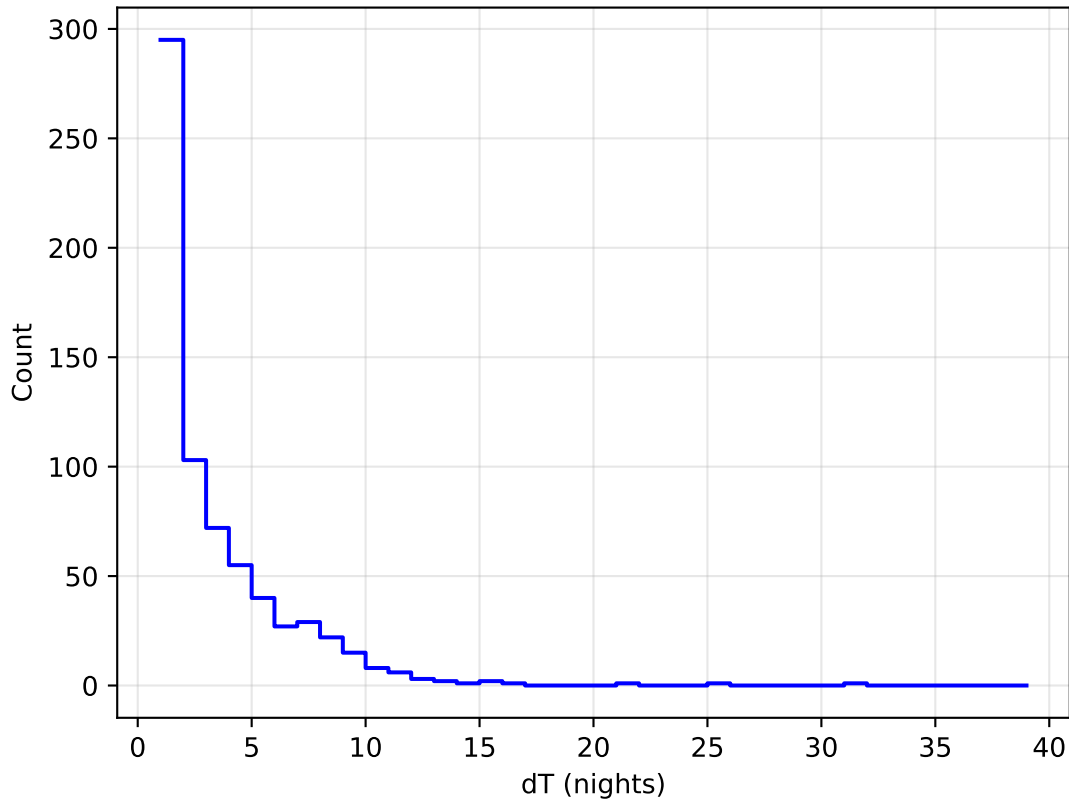
ddf_loaded_fl15_v3.4_10yrs all bands: DD:ELAISS1 Delta Nights Histogram
