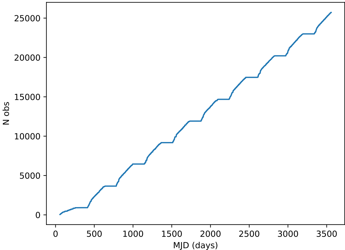
ddf_loaded_fl15_v3.4_10yrs all bands: DD:ELAISS1 Cumulative NVisits
