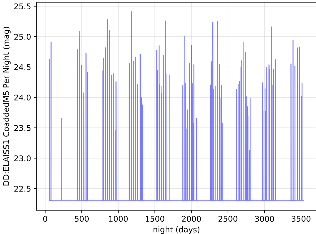
ddf_loaded_fl15_v3.4_10yrs u band: DD:ELAISS1 CoaddedM5 Per Night
