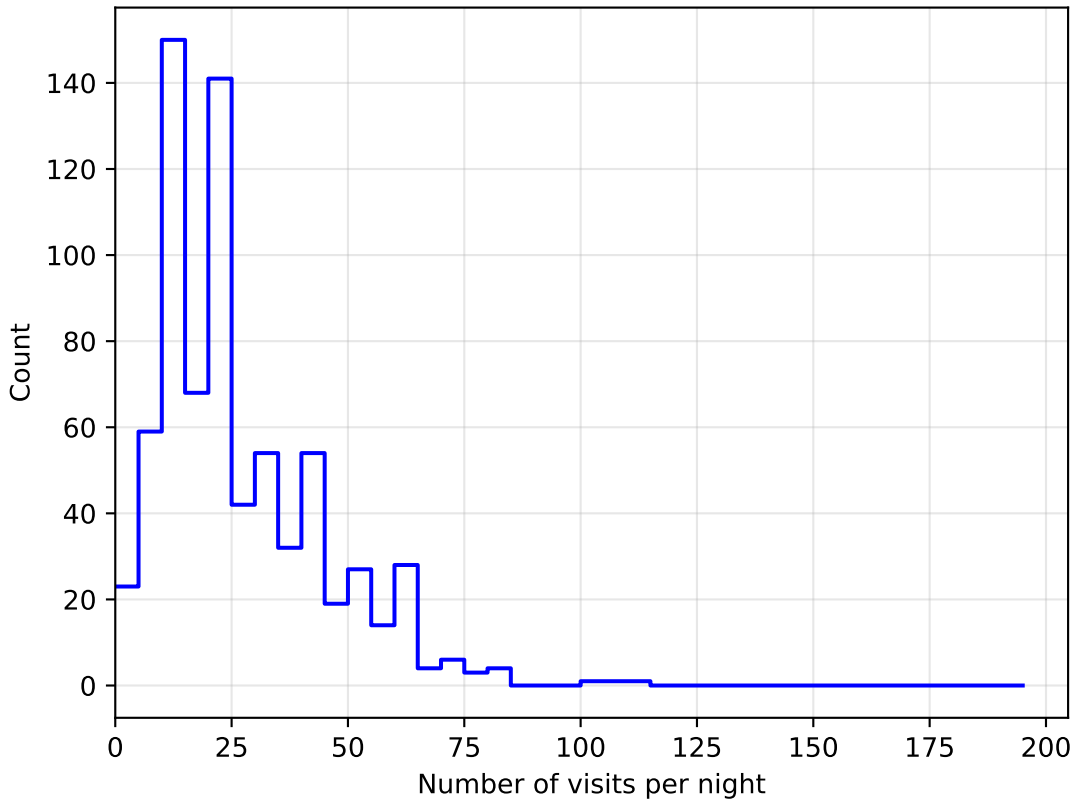
ddf_loaded_fl15_v3.4_10yrs all bands: DD:EDFS NVisitsPerNight
