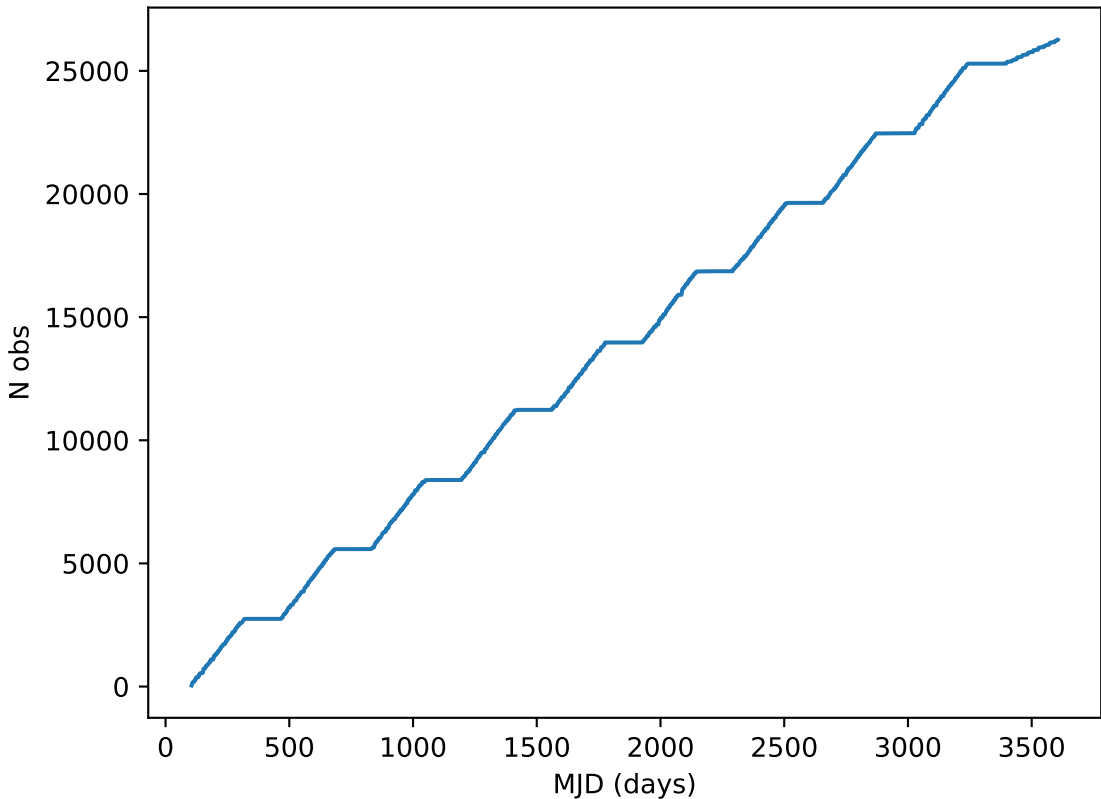
ddf_loaded_fl15_v3.4_10yrs all bands: DD:EDFS Cumulative NVisits
