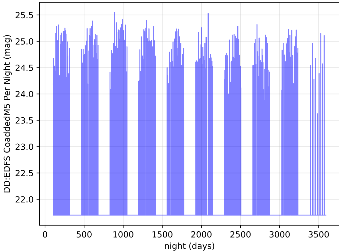
ddf_loaded_fl15_v3.4_10yrs z band: DD:EDFS CoaddedM5 Per Night
