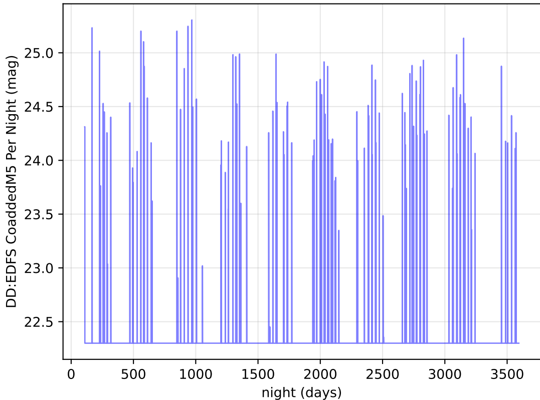
ddf_loaded_fl15_v3.4_10yrs u band: DD:EDFS CoaddedM5 Per Night
