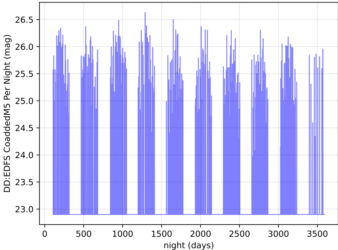
ddf_loaded_fl15_v3.4_10yrs r band: DD:EDFS CoaddedM5 Per Night
