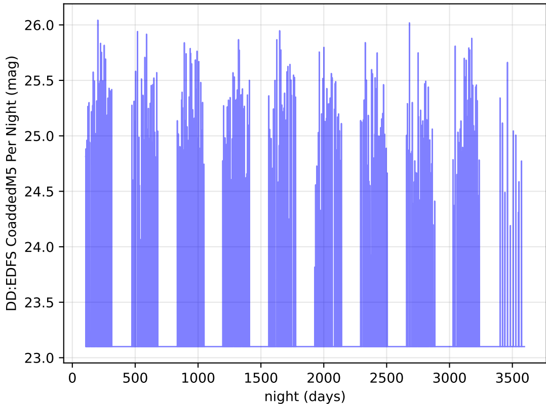
ddf_loaded_fl15_v3.4_10yrs i band: DD:EDFS CoaddedM5 Per Night
