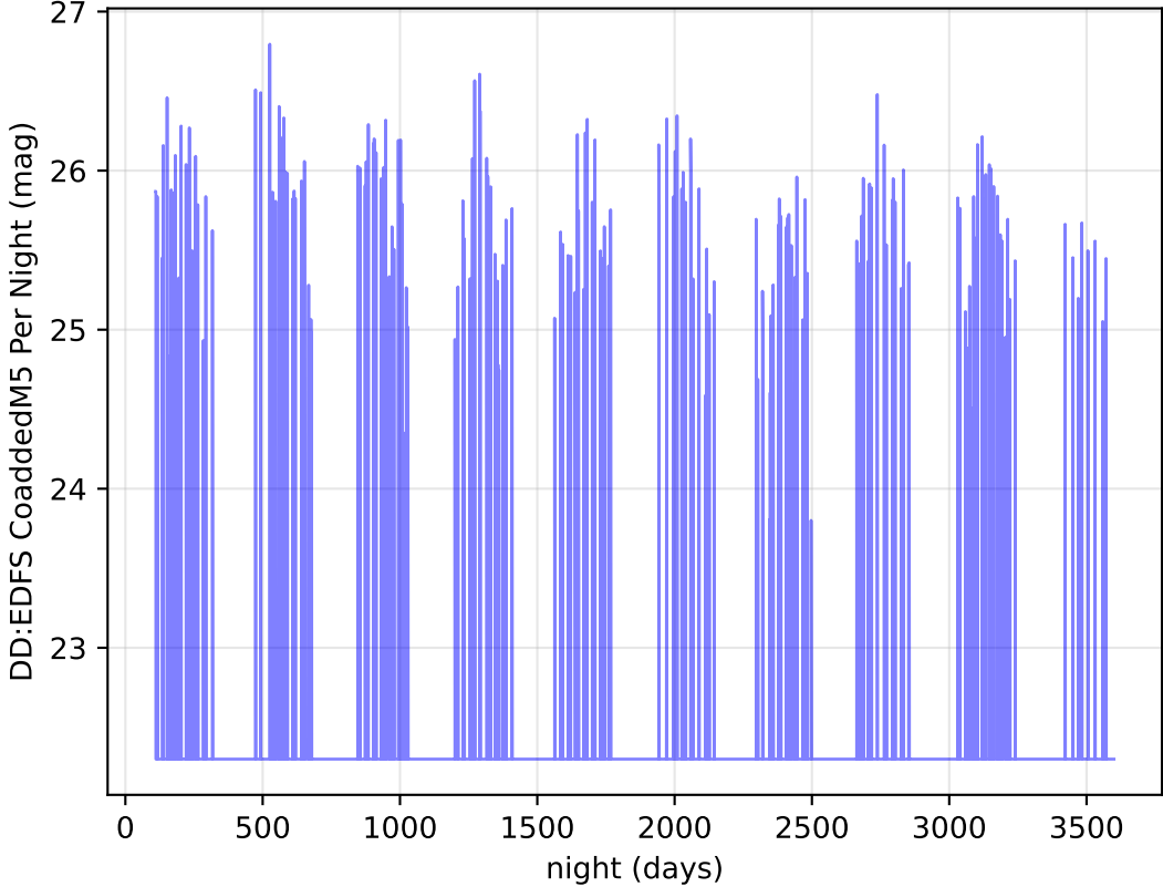
ddf_loaded_fl15_v3.4_10yrs g band: DD:EDFS CoaddedM5 Per Night
