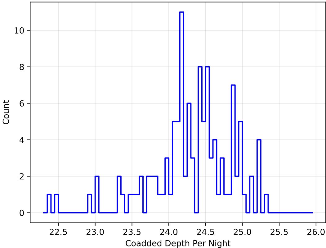
ddf_loaded_fl15_v3.4_10yrs u band: DD:EDFS CoaddM5PerNight
