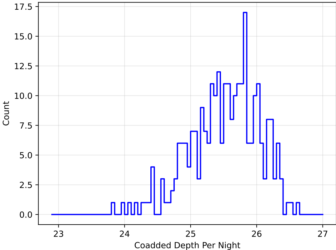
ddf_loaded_fl15_v3.4_10yrs r band: DD:EDFS CoaddM5PerNight
