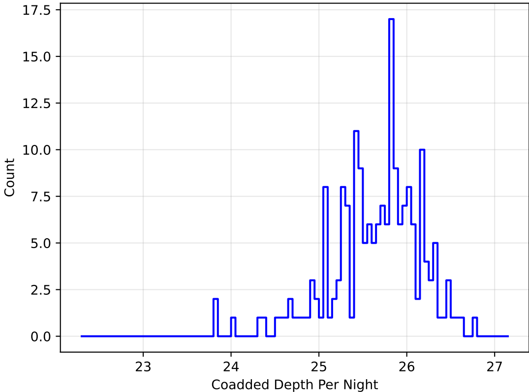
ddf_loaded_fl15_v3.4_10yrs g band: DD:EDFS CoaddM5PerNight
