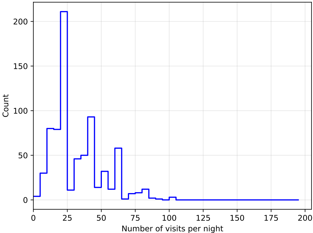
ddf_loaded_fl15_v3.4_10yrs all bands: DD:ECDFS NVisitsPerNight
