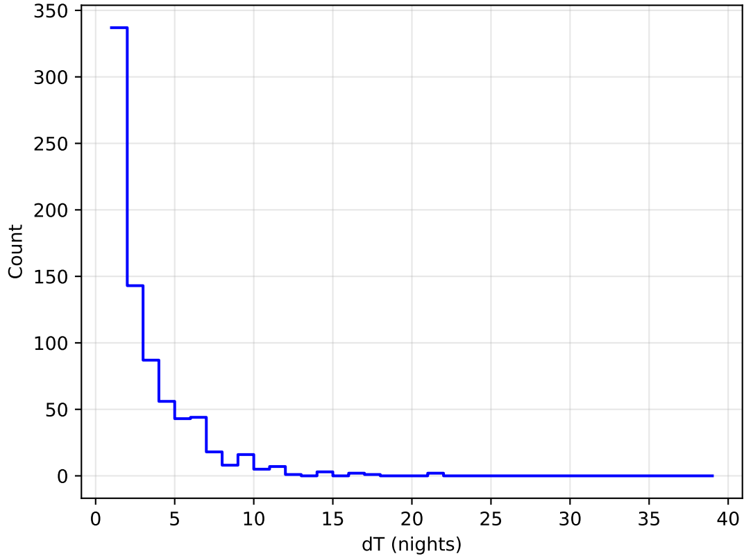
ddf_loaded_fl15_v3.4_10yrs all bands: DD:ECDFS Delta Nights Histogram
