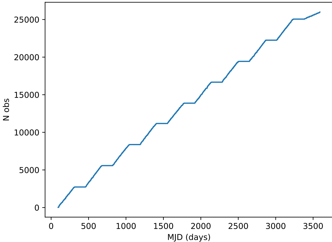
ddf_loaded_fl15_v3.4_10yrs all bands: DD:ECDFS Cumulative NVisits
