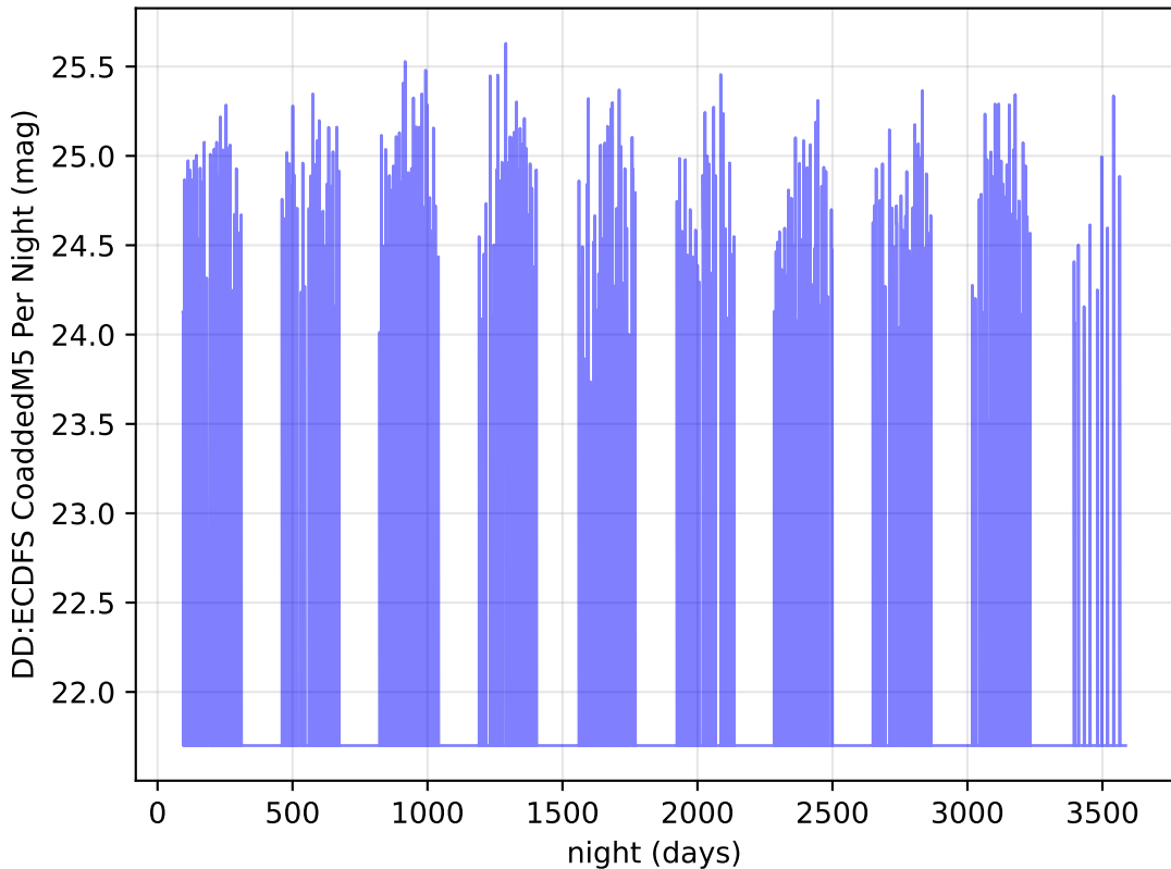
ddf_loaded_fl15_v3.4_10yrs z band: DD:ECDFS CoaddedM5 Per Night
