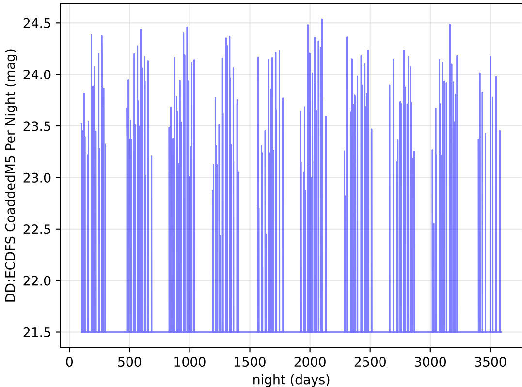
ddf_loaded_fl15_v3.4_10yrs y band: DD:ECDFS CoaddedM5 Per Night
