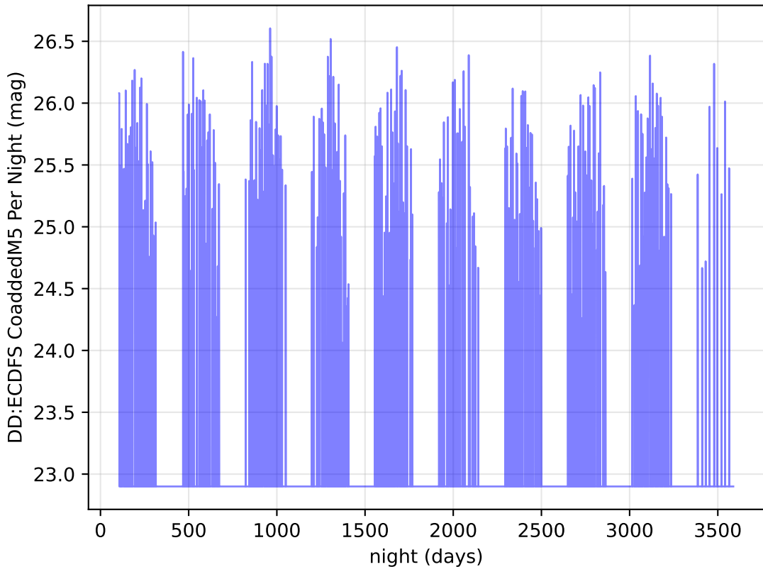
ddf_loaded_fl15_v3.4_10yrs r band: DD:ECDFS CoaddedM5 Per Night
