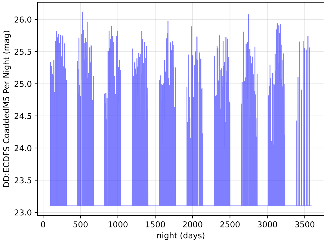
ddf_loaded_fl15_v3.4_10yrs i band: DD:ECDFS CoaddedM5 Per Night
