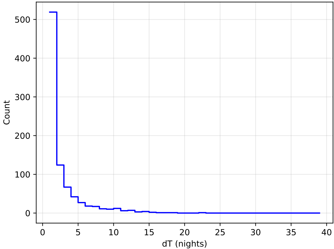
ddf_loaded_fl15_v3.4_10yrs all bands: DD: COSMOS Delta Nights Histogram
