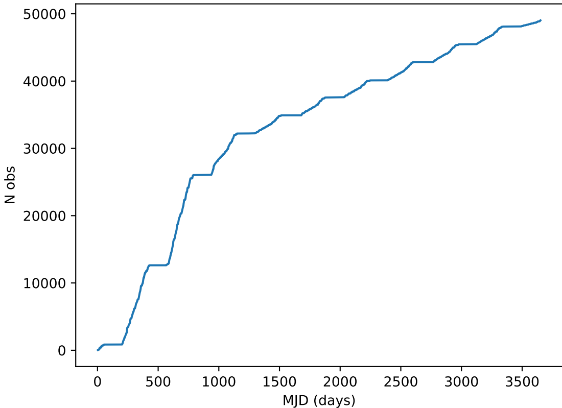
ddf_loaded_fl15_v3.4_10yrs all bands: DD: COSMOS Cumulative NVisits
