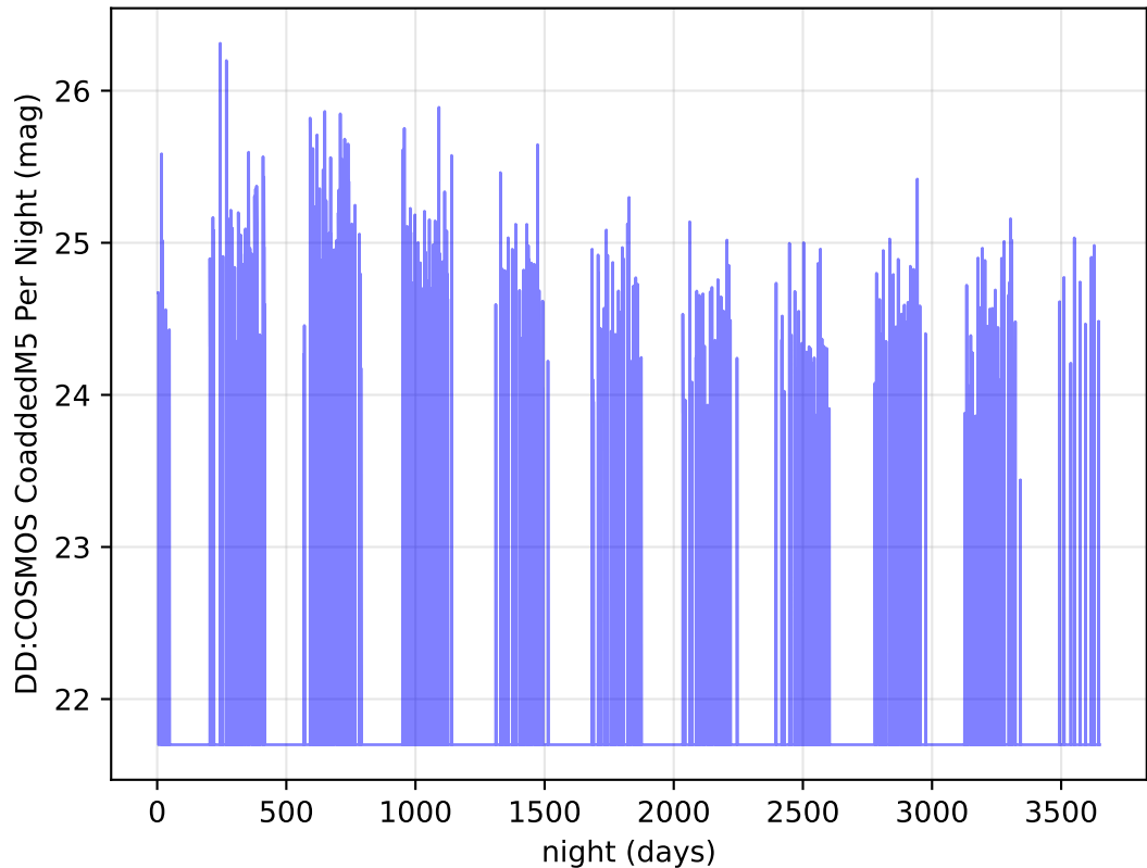
ddf_loaded_fl15_v3.4_10yrs z band: DD:COSMOS CoaddedM5 Per Night
