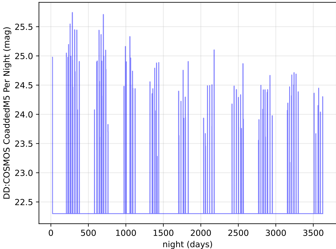
ddf_loaded_fl15_v3.4_10yrs u band: DD:COSMOS CoaddedM5 Per Night
