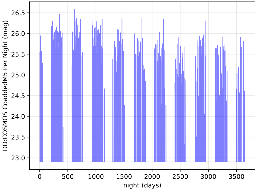
ddf_loaded_fl15_v3.4_10yrs r band: DD:COSMOS CoaddedM5 Per Night
