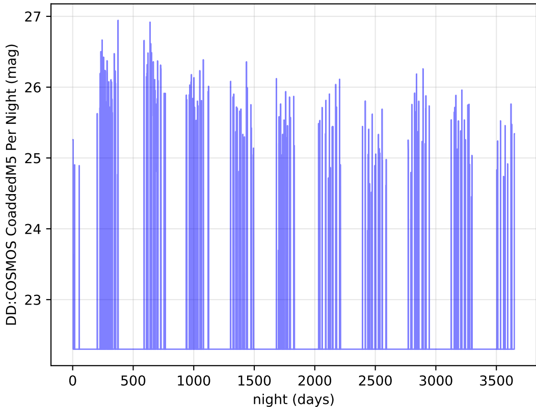
ddf_loaded_fl15_v3.4_10yrs g band: DD:COSMOS CoaddedM5 Per Night
