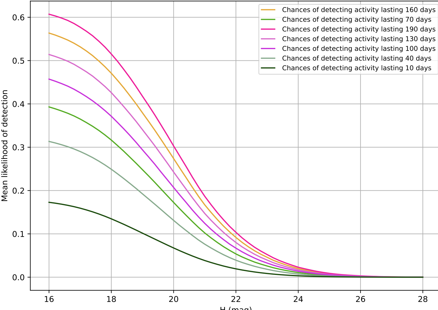
ddf_half_v3.4_10yrs PHA
